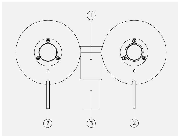
Figure 3 Top view of RA01: (1) leveling assembly for x- and y-axis, (2) cables, (3) mounting tube (not included).
