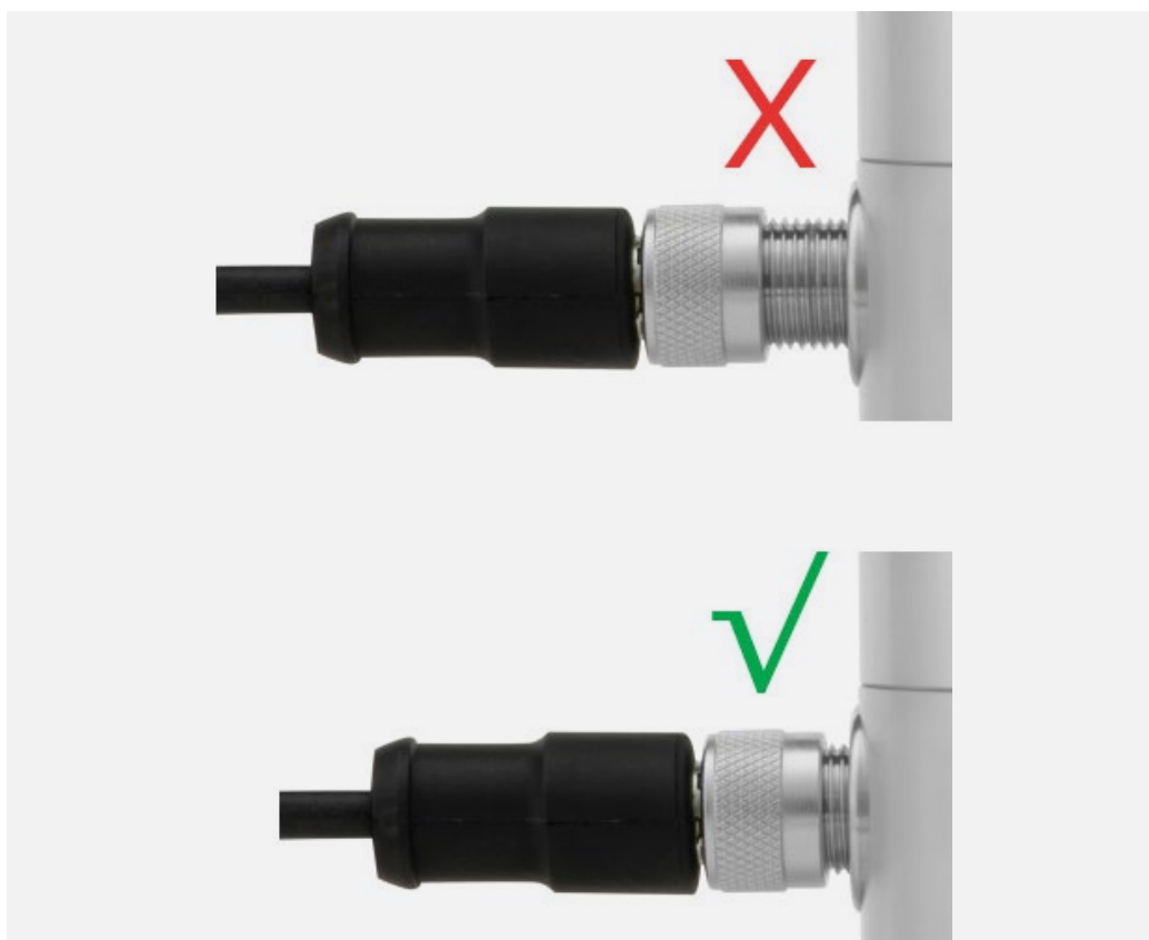
Figure 5.3.4.1 Connection of the cable connector to the chassis connector: make sure to completely tighten the screw lock. This is necessary for proper sealing against moisture and proper electrical connection of conductors and cable shield.
