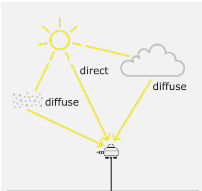
Figure 2.1.1 Diffuse solar radiation is defined as all solar radiation reaching the surface that does not come directly from the sun. It may come from solar radiation scattered by clouds, atmospheric particles, and aerosols.
