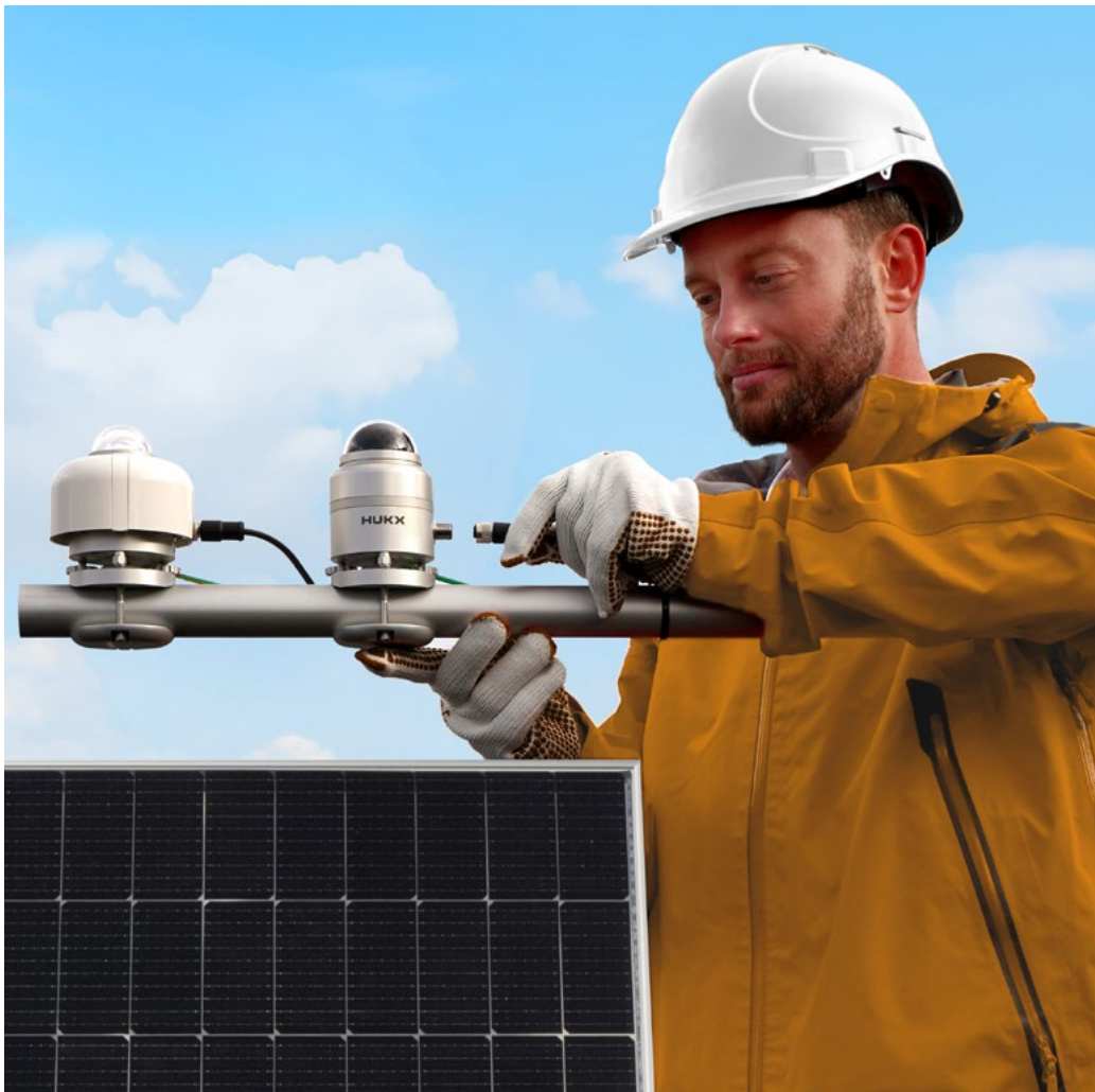
Figure 0.3 Typical installation of SRD100-D1, next to a normal Class A pyranometer, such as the SR300-D1.
