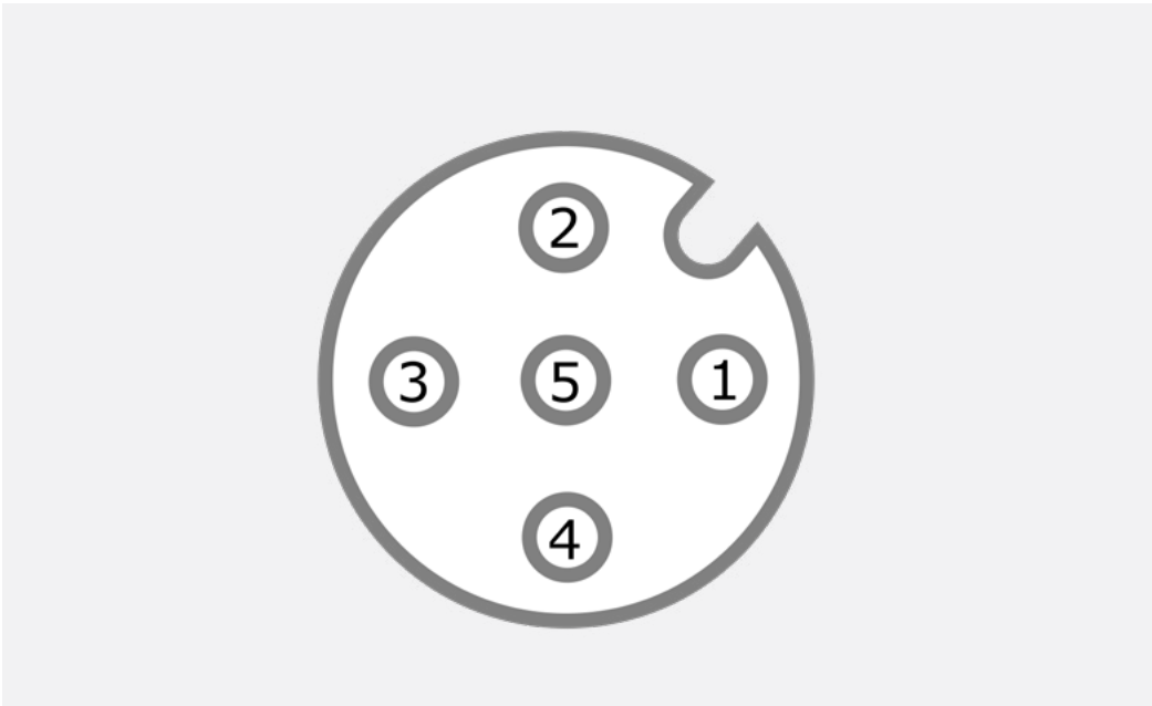
Figure 5.5.1 Schematic of the M12-A connector layout of Hukx industrial instruments, indicating the PIN numbers.
