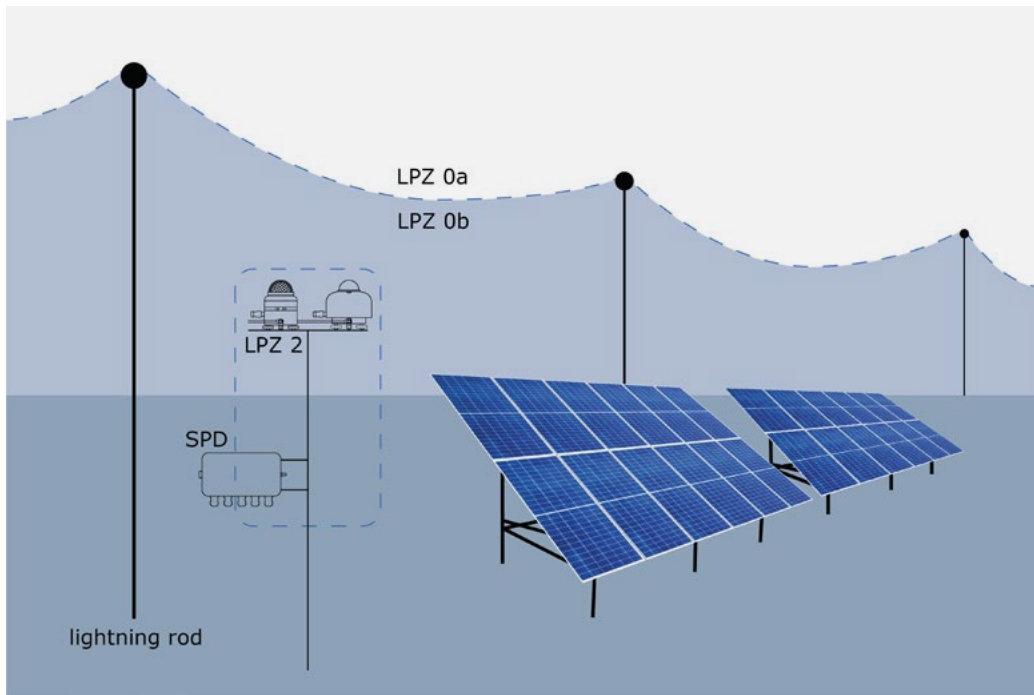
Figure 5.4.1.1 Hukx industrial instruments, including SRD100-D1, should be installed in LPZ2. Hukx SPD01 is a type 2 SPD which is used on the zone boundary from LPZ0b to LPZ2.
