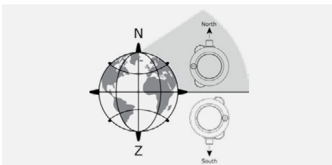
Figure 5.1.2 By convention, when installing the pyranometer in a horizontal orientation, the connector should be pointing north on the northern hemisphere and south on the southern hemisphere.
