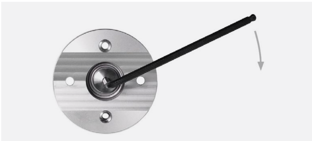
Figure 5.3.4.1.2 Bottom of LM01 leveling mount. Preferred (un) locking with 4 mm hex key.
