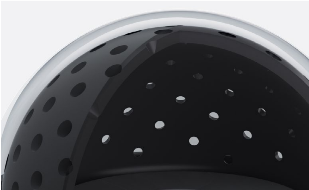
Figure 2.2.1 Schematic illustration of the SRD100-D1 working principle. The SRD100-D1 D1 diffusometer features a sensor array and half-sphere shadow mask above the array with a unique Fibonacci lattice hole pattern. All sensors are centrally located under the mask, ensuring that at least one sensor remains in the shade. This shaded sensor is near-homogeneously exposed only to diffuse sky, giving an accurate estimate of diffuse solar irradiance.
