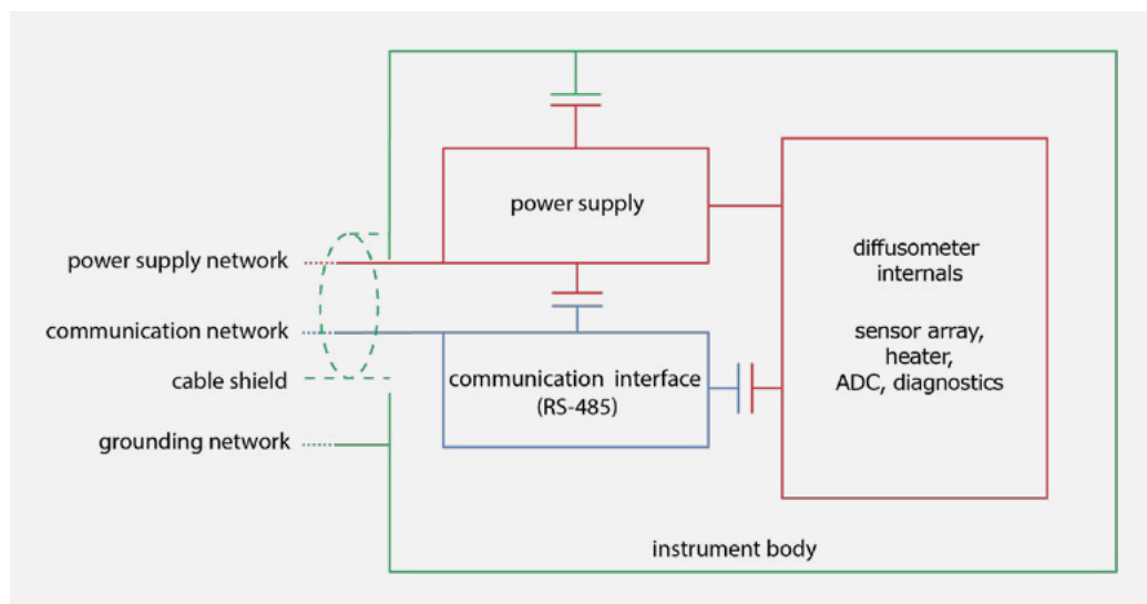
Figure 5.4.5.1 Schematic representation of industrial instruments indicating the electrical connections and the different isolation barriers.
