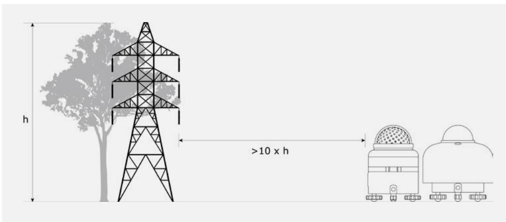
Figure 5.1.1 Preferably, the field of view of the diffusometer should be unobstructed by nearby obstacles. If obstructions are present, as a rule of thumb the diffusometer should be installed at least 10 times the height of the obstruction away from the obstruction.
