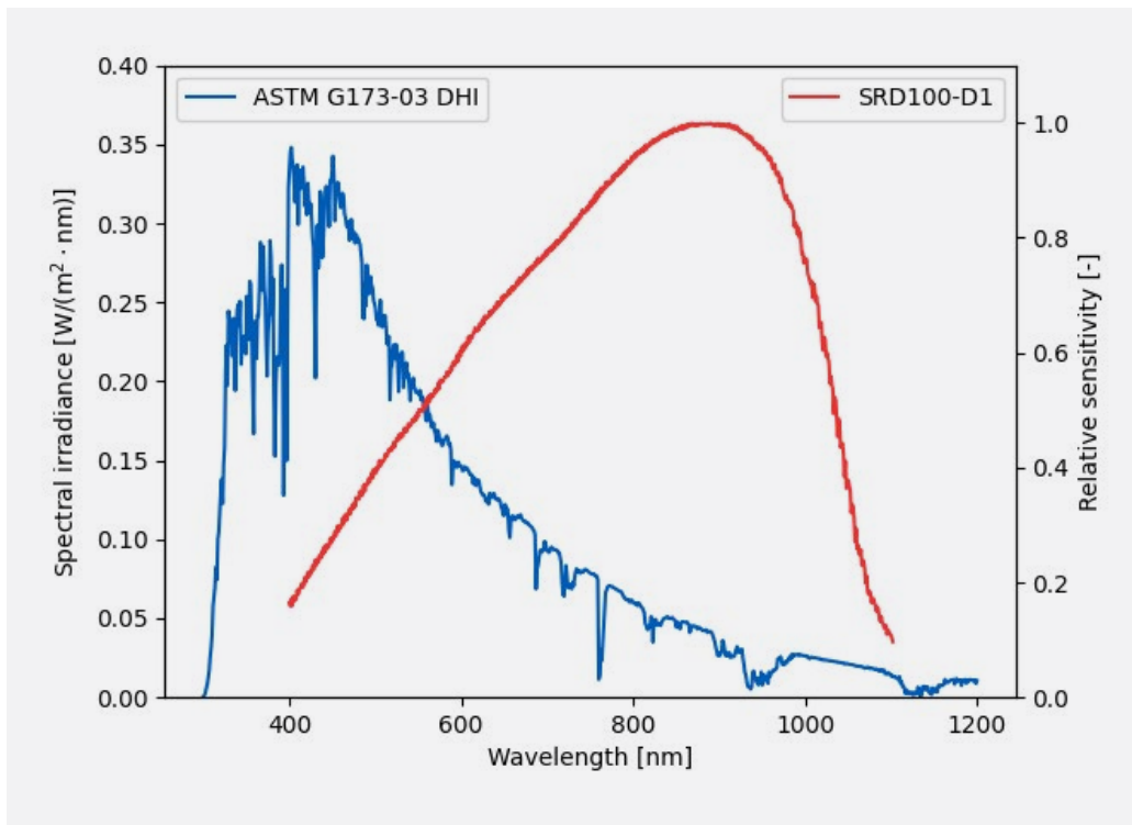
Figure 8.7.1.1 The ASTM G173-03 diffuse horizontal equivalent spectrum and the spectral sensitivity of the SRD100-D1.
