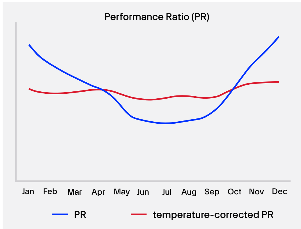
Figure 2.3.1. Performance Ratio (PR) with and without temperature correction. This schematic graph is for a PV system located in the northern hemisphere. Temperature measurements with PVMT01 can be used for temperature correction.
