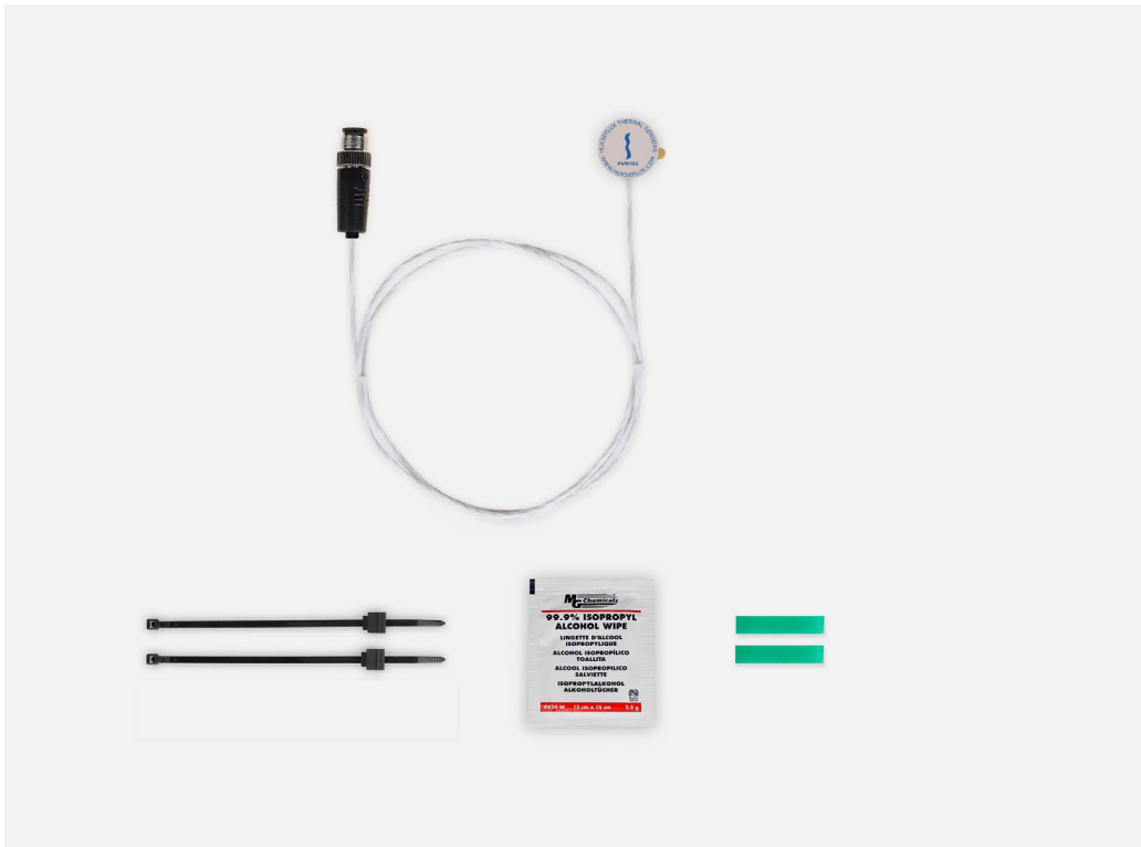
Figure 1.2.1 PVMT01 comes with 2 x solar clips, 2 x polyester tapes and a pre-saturated IPA wipe.
