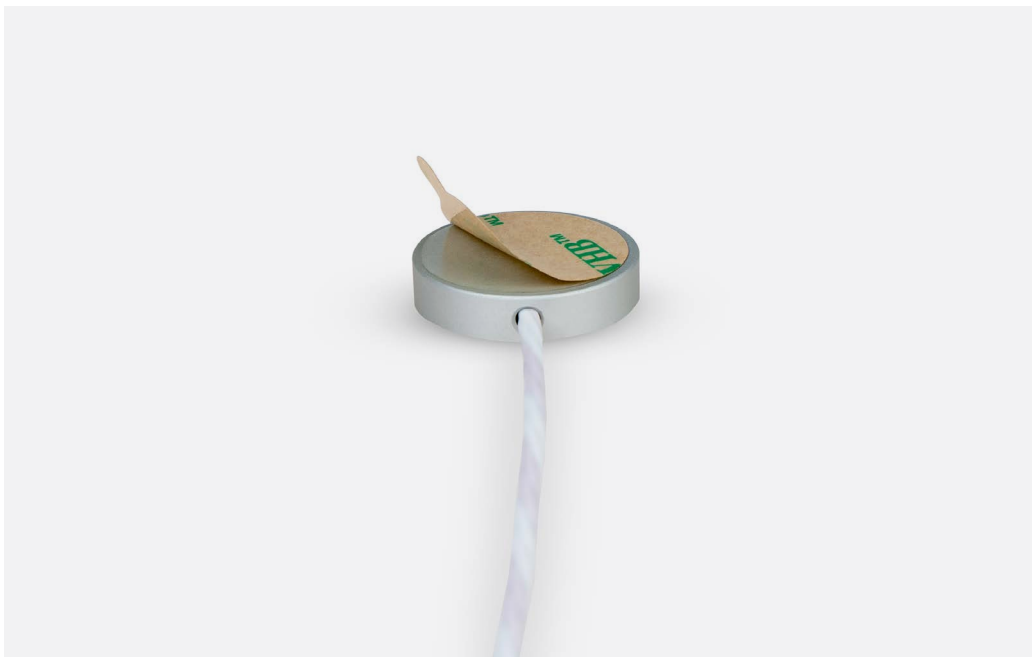
Figure 2.1.1 Adhesive on the back of the aluminum disk with excellent thermal properties. The paper release liner should be removed before mounting the sensor to the surface.
