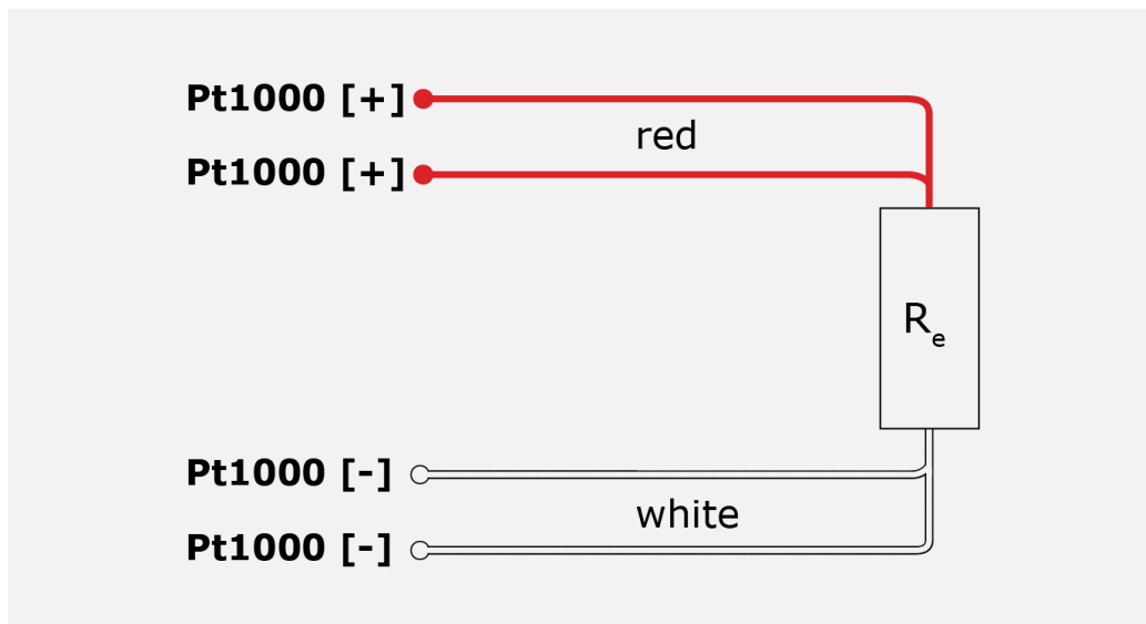
Figure 4.4.1. 2-wire circuit diagram, R_e represents the sensor resistance.
