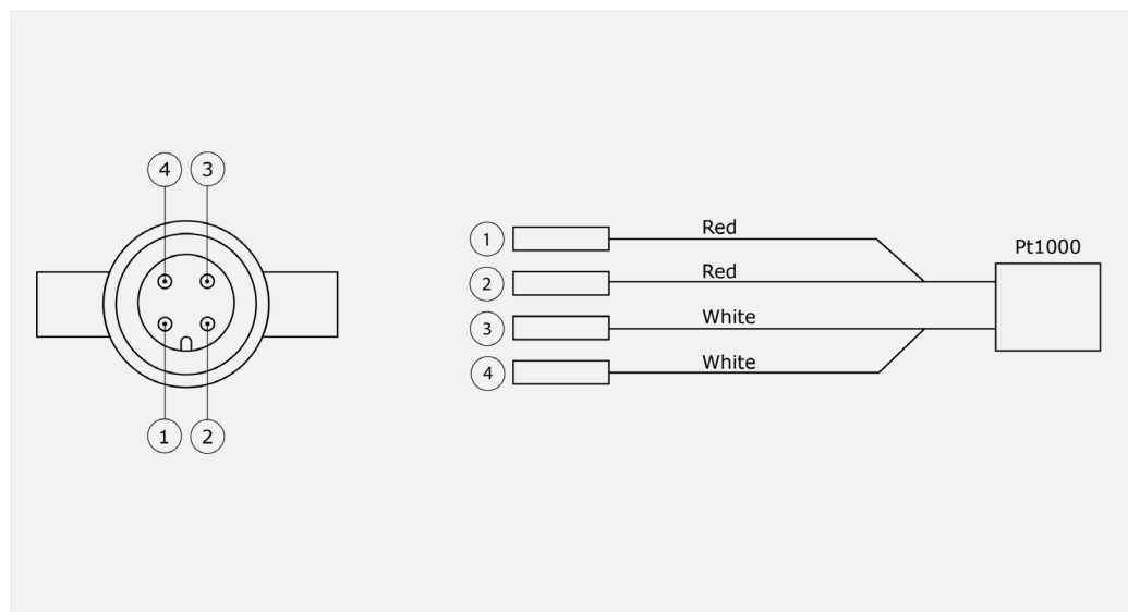
Figure 4.2.1. Schematic PVMT01 4P M12 connector diagram, indicating the pin numbers.
