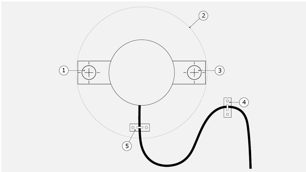
Figure 5.1.1 Installation of HF05
