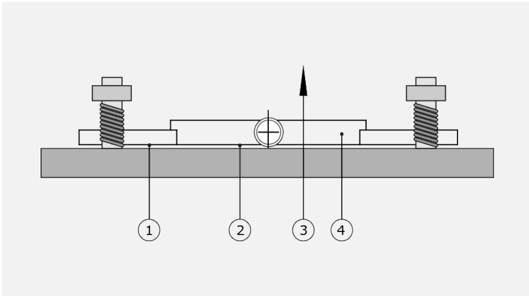
Figure 5.1.3 1. engraved serial number 2. HF05 side of object to be measured, flush with flanges 3. heat flux generating positive signal 4. engraved with marker 'X'
