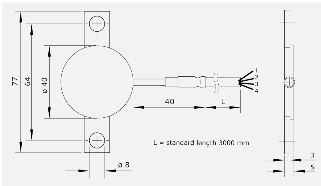
Figure 3.2.1 HF05 heat flux sensor dimensions in \times 10^{-3} \text{ m} .
