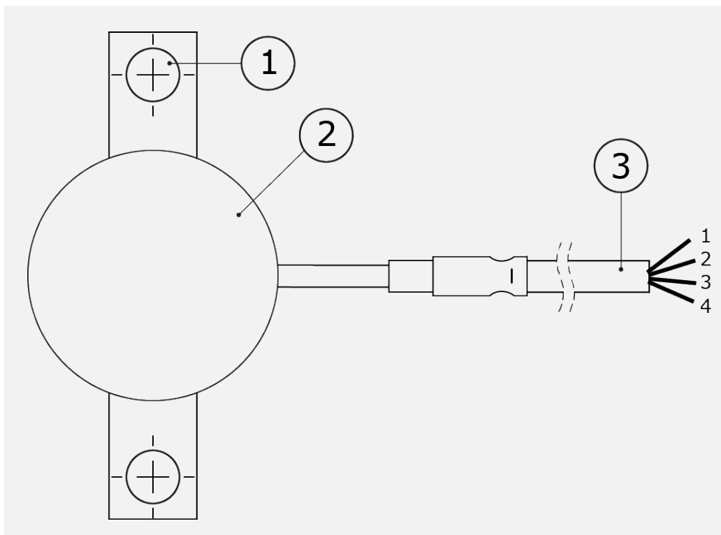
Figure 2.2 HF05: the heat flux sensor (2) is connected to a short rigid stainless-steel tube. This sensor-to-cable transition is connected to a PTFE cable (3). Two mounting flanges (1) are attached to the sensor body.
