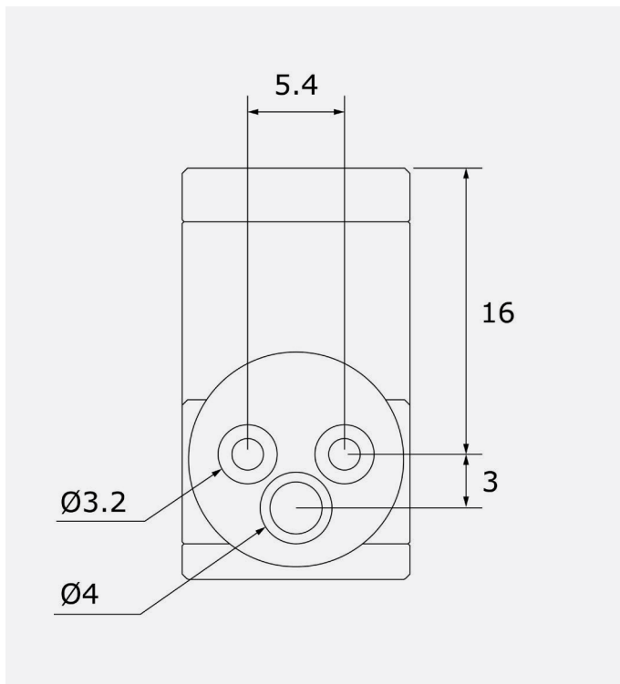
Figure 5.2.2 Dimensions for cone calorimeter mounting, sensitive area to cooling tubes center 16 mm.
