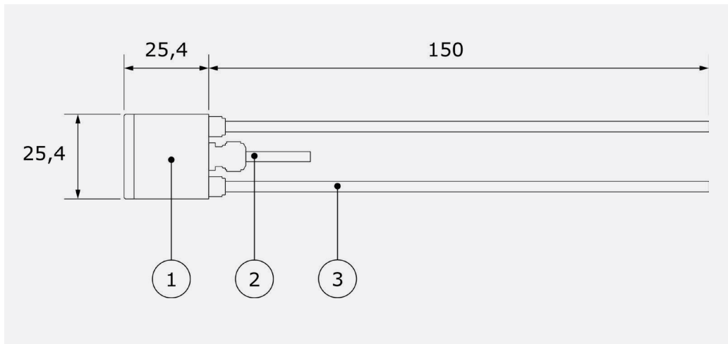
Figure 3.3.1 SGB03-010-02-P150 heat flux sensor with a smooth body, side view dimensions in \times 10^{-3} \text{ m} .
