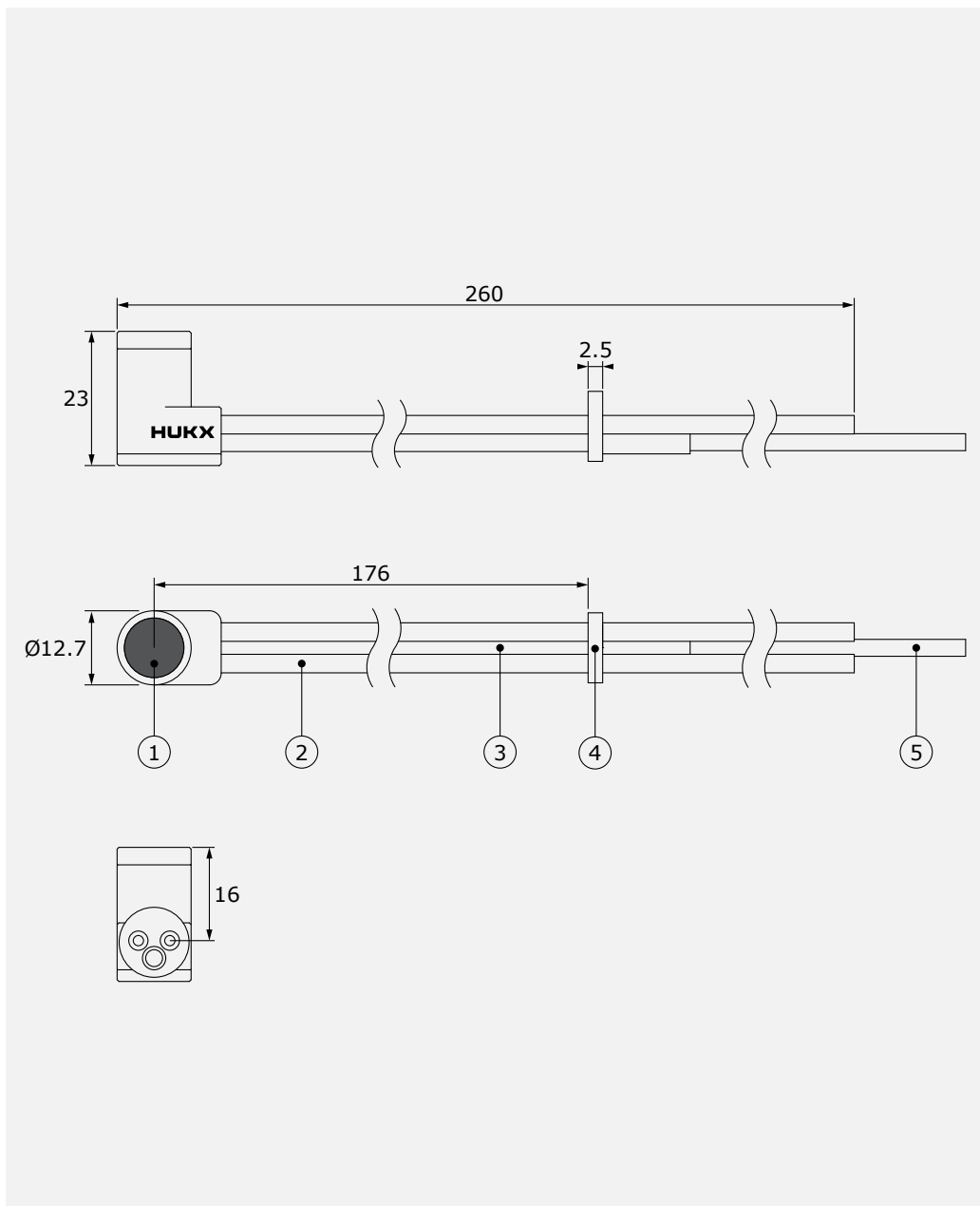
Figure 3.4.1 SGB04 heat flux sensor, dimensions in \times 10^{-3} \text{ m} . From top to bottom: front view, top view, side view
