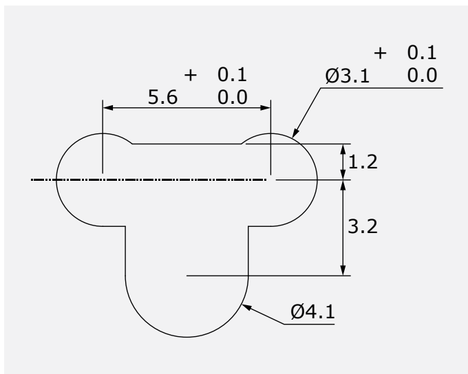
Figure 5.2.3 Suggested slot dimensions for SBG04 cone calorimeter "Flux meter mount".
