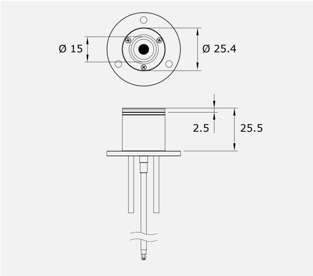
Figure 3.3.1 GG01 with sapphire window, dimensions in 10^{-3} \text{ m} . The window is added to a standard GG01. GG01s with sapphire window (GG01-250-SW) are custom made, the sapphire window cannot be used on a standard GG01. For other dimensions, see previous section on GG01 dimensions.
