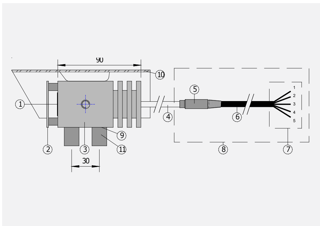
Figure 2 HF02 consists of a heat flux sensor (1) providing both a heat flux and a sensor body temperature measurement, a sensor body (3), a radiation shield (2) and rain screen (10) to protect the sensor against the environment, a high-temperature metal-sheathed cable (4), a cable transition piece (5), a low-temperature extension cable (6), mounting holes (3/8 UNC) (9) and spacers (11). The transition piece (5) to the cable end (at 7) in area 8 must be between -20 and +70^\circ\text{C} , and the cable end (at 7) must be provided by the user with an enclosure certified for use in the area of installation. Installation is the responsibility of the user. Dimensions in \times 10^{-3} \text{ m} .
